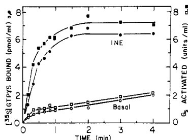
FIGURE 1: Agonist-stimulated activation of G_s and stable [ ^{35}\text{S} ]GTP \gamma S binding in receptor- G_s vesicles. Vesicles were incubated at 30 °C in medium containing 0.1 \mu\text{M} [ ^{35}\text{S} ]GTP \gamma S, 2 mM \text{MgCl}_2 , 1 mM EDTA, and either 100 nM (—)propranolol (open symbols) or 1 \mu\text{M} (—)isoproterenol. At the times indicated, aliquots were withdrawn into two volumes of quenching solution and assayed for activation of G_s by reconstitution with \text{cyc}^+ membranes ( \square , \blacksquare ) or for [ ^{35}\text{S} ]GTP \gamma S bound ( \circ , \bullet ) as described under Experimental Procedures. The incremental effects due to isoproterenol are shown by the solid symbols. Data are expressed according to the volume of vesicles used for each assay. The concentration of reconstituted receptors in this experiment was 1.2 nM.
