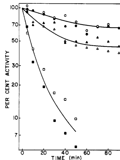
FIGURE 3: Comparison of G_s activation and [ ^{35}\text{S} ]GTP \gamma S binding: The stability of reconstituted G_s . Vesicles were incubated at 30 °C in 20 mM NaHepes (pH 8), 0.1 M NaCl, 1 mM dithiothreitol, 0.1 mM ascorbate, and 1 mM EDTA, plus either 2 mM \text{MgCl}_2 ( \blacktriangle , \triangle ), 2 mM \text{MgCl}_2 plus 1 \mu\text{M} (—)isoproterenol ( \circ , \bullet ), or 50 mM \text{MgCl}_2 ( \blacksquare , \square ). At the indicated times, aliquots were withdrawn and incubated with 0.1 \mu\text{M} [ ^{35}\text{S} ]GTP \gamma S, 10 \mu\text{M} (—)propranolol, and 50 mM \text{MgCl}_2 for 14 min at 30 °C. The reaction was terminated by addition of quenching solution, and the reaction mixture was assayed both for [ ^{35}\text{S} ]GTP \gamma S bound (open symbols) and for G_s activation (closed symbols). The binding of GTP \gamma S at zero time was 2.5 ( \circ ), 2.4 ( \triangle ), and 1.8 pmol/mL ( \square ). The reconstitutive G_s activity at zero time was 2.1 ( \bullet ), 2.0 ( \blacktriangle ), and 1.4 units/mL ( \blacksquare ).
