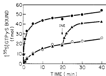
FIGURE 2: Continued responsiveness of receptor- G_s vesicles to stimulation by agonist. Vesicles were incubated at 30 °C with 100 nM [ ^{35}\text{S} ]GTP \gamma S and 1 mM free \text{Mg}^{2+} in the presence ( \bullet ) or absence ( \circ , \blacktriangle ) of 10 \mu\text{M} (—)isoproterenol. At the times shown, 25- \mu\text{L} aliquots were assayed for bound [ ^{35}\text{S} ]GTP \gamma S. At 20 min, isoproterenol (INE) (10 \mu\text{M} final) was added to one sample ( \blacktriangle ). Each 25- \mu\text{L} aliquot contained 18 fmol of receptor.
